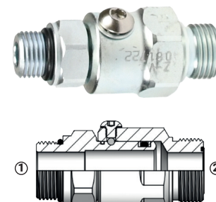
(1) Macho ORB (2) Macho Face Seal
